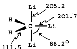
(17) C_{2v}
