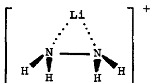
(55) C 2v
