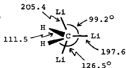
(26) C_{2v}
