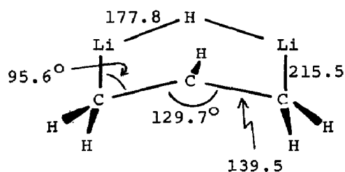
(49) C s
