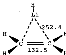
(50) C 2v
