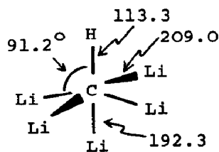
(20) C_{4v}
