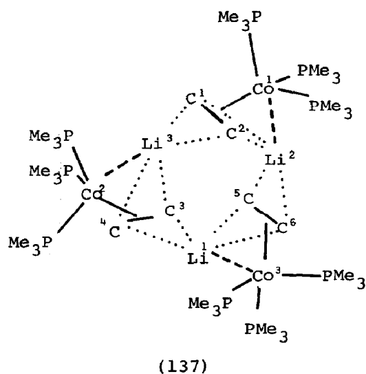
Bond distances/pm in (137)
