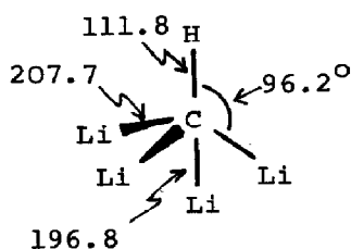
(16) C_{3v}
