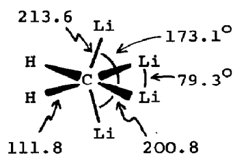
(21) C_{2v}
